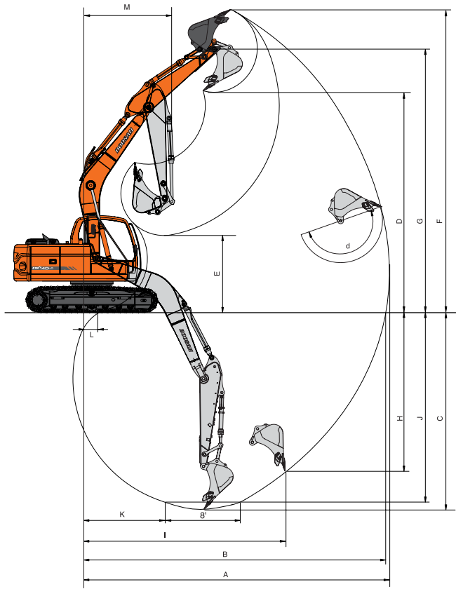
[ One-piece Boom ]
